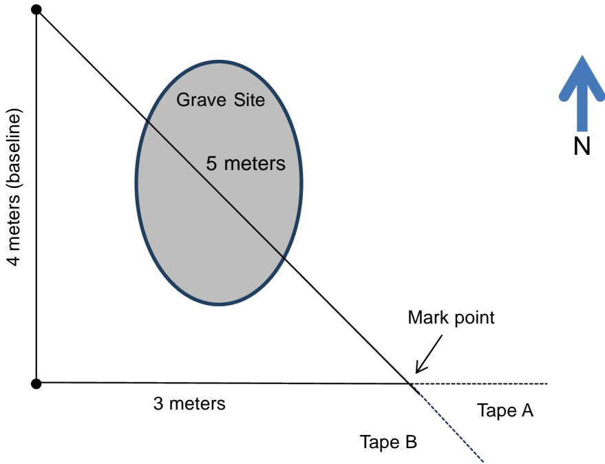
Figure : 3 Setting limits and datum for mapping (Set up of a 3-4-5 triangle)
