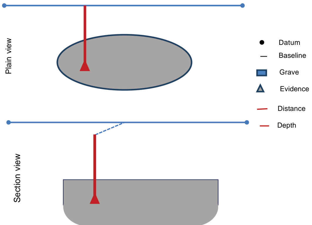
Figure : 4 Method of baseline perpendicular measurement
