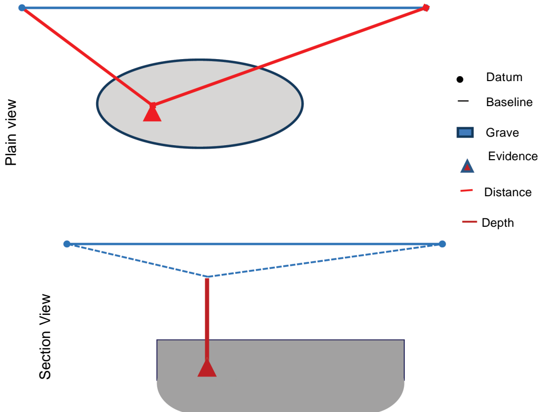
Figure : 6 Method of baseline triangulation measurement
