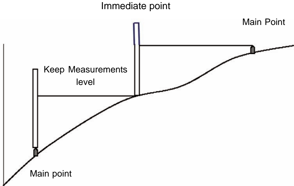
Figure : 5 Use of intermediate datum points when mapping on a slope
